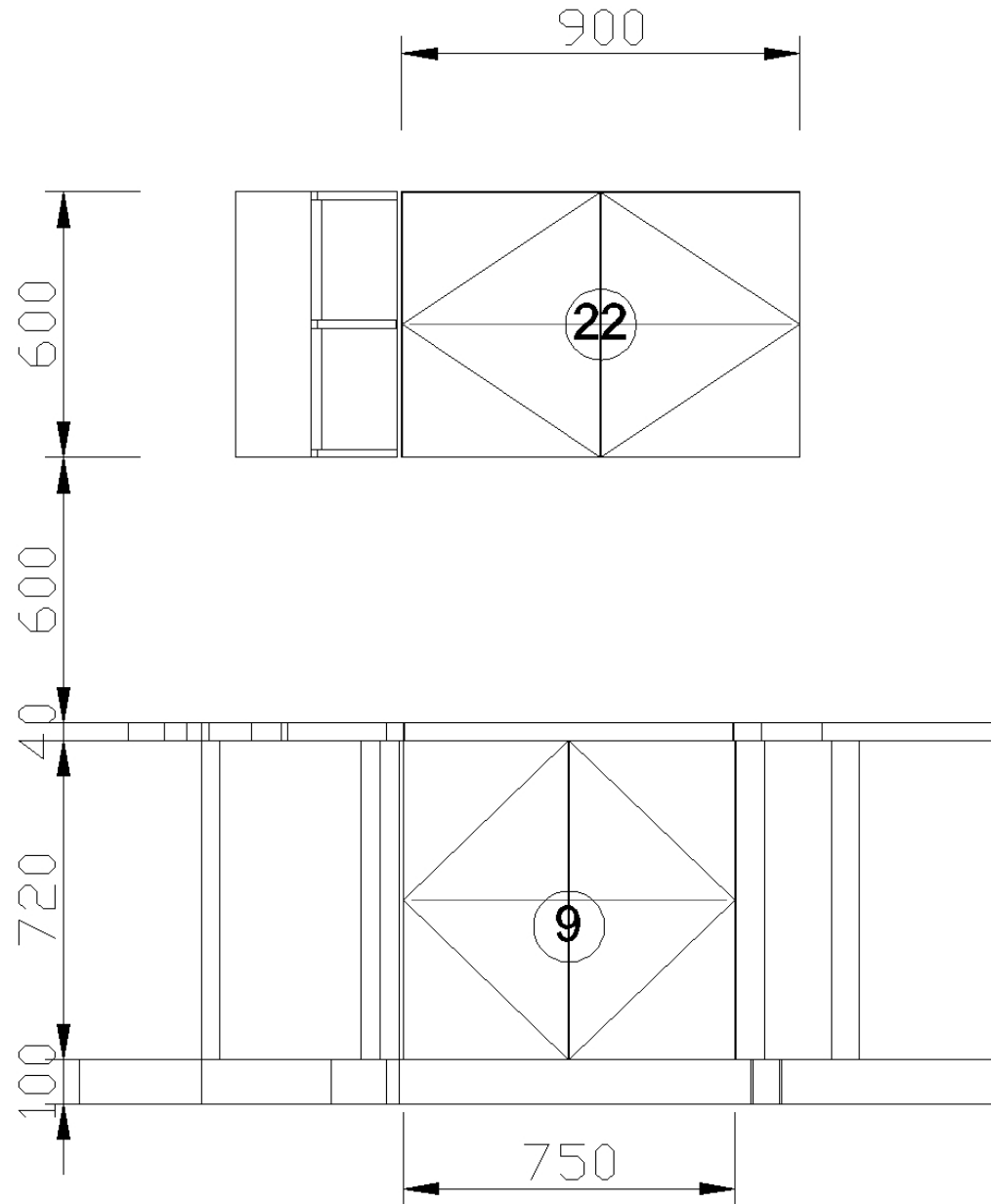
J View elevation drawing
