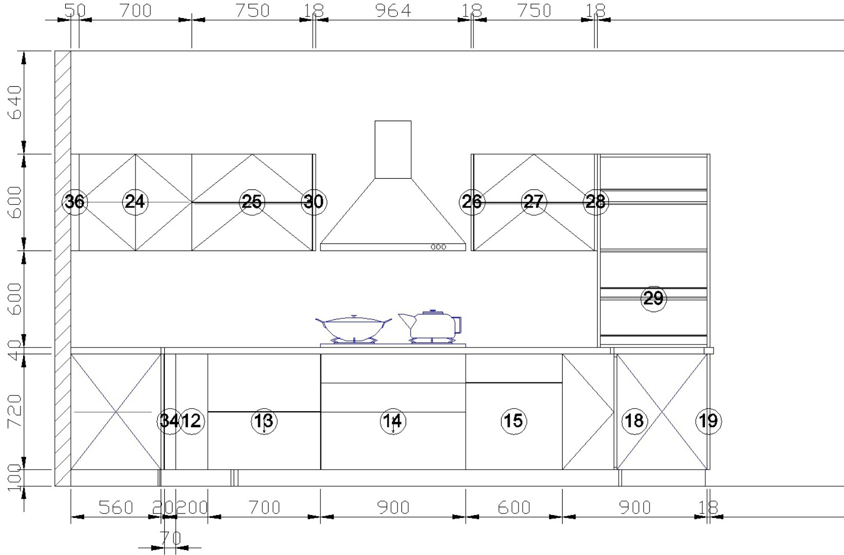
E View elevation drawing
