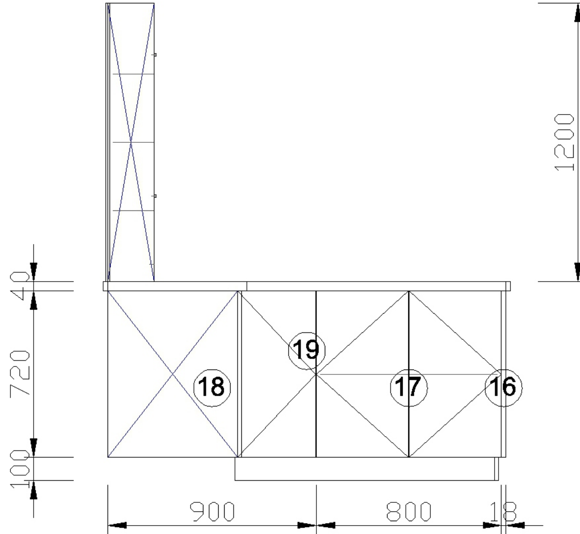
G View elevation drawing
